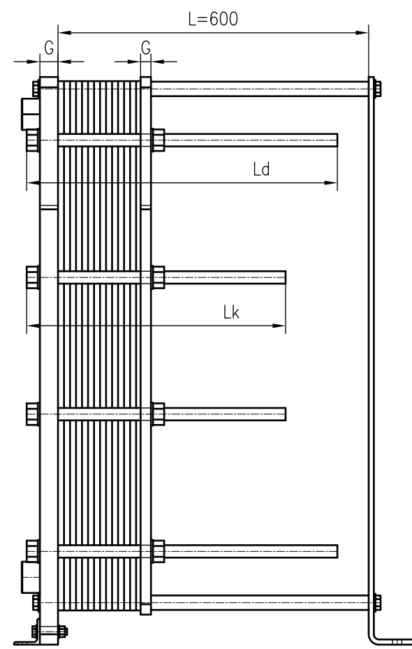
Side view
