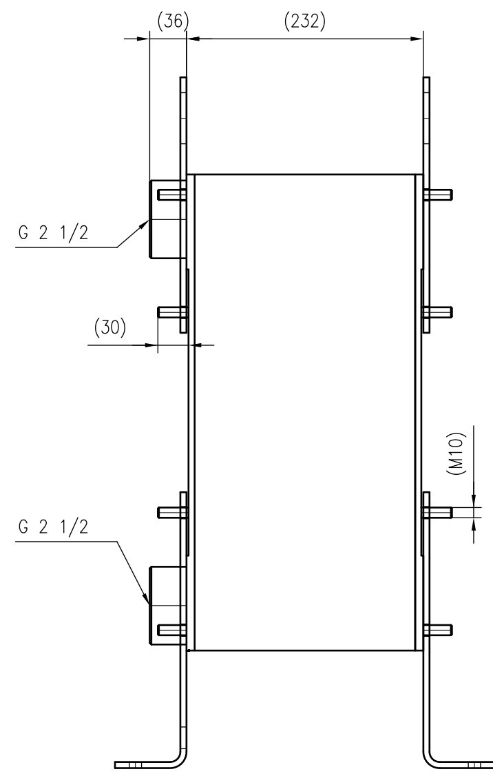
Side view
