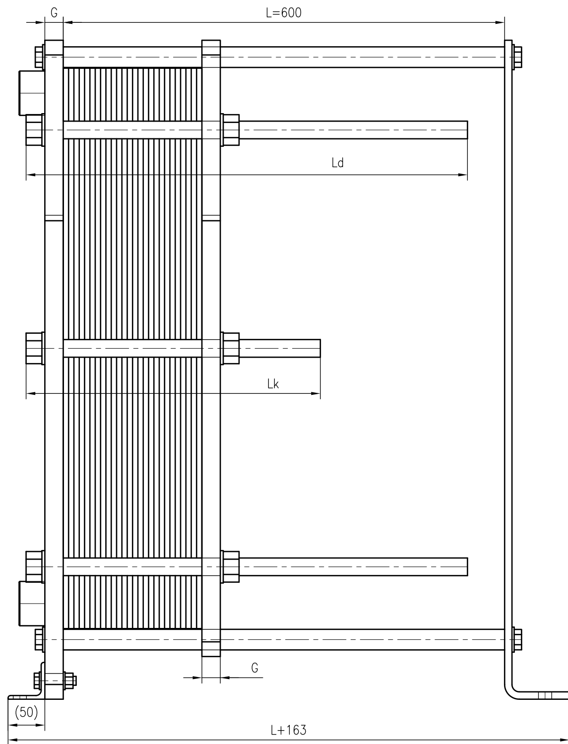
Side view
