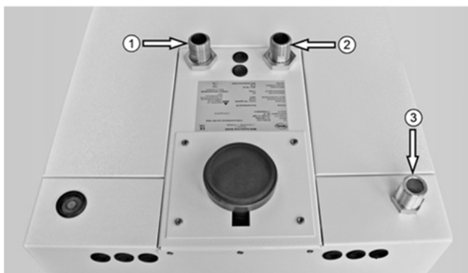
Abb. 11: Kesselanschlüsse
