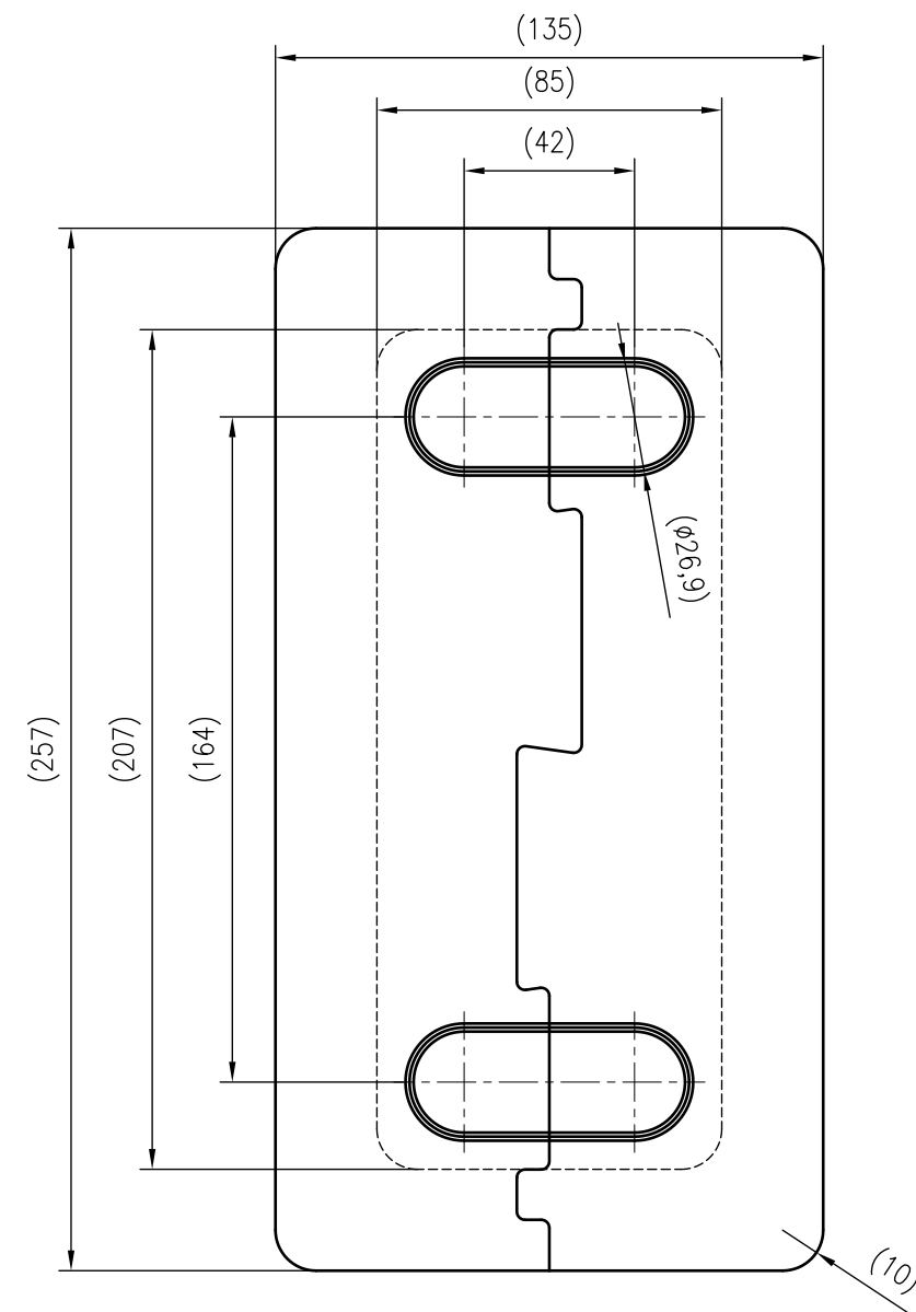
Front view
