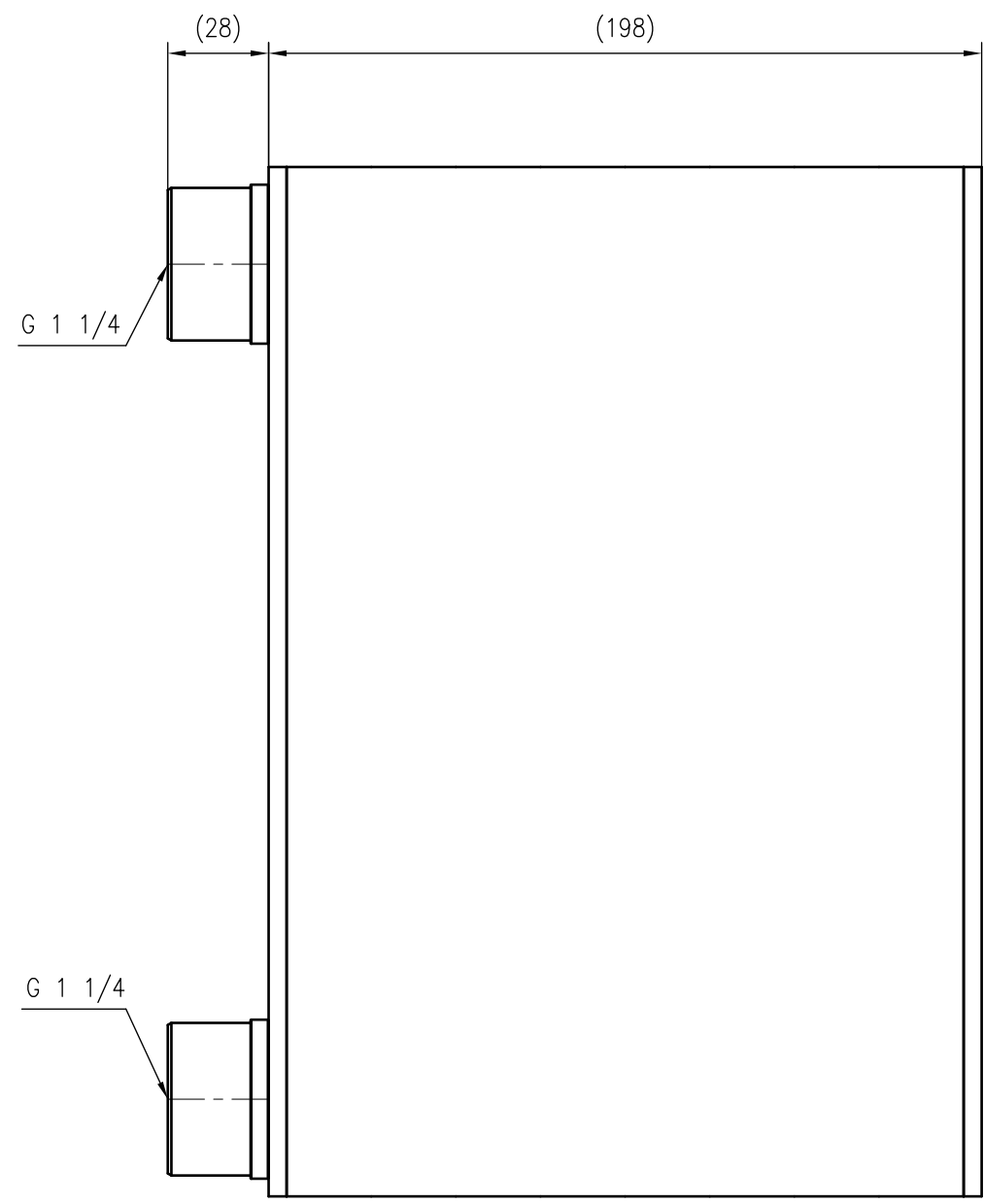
Side view
