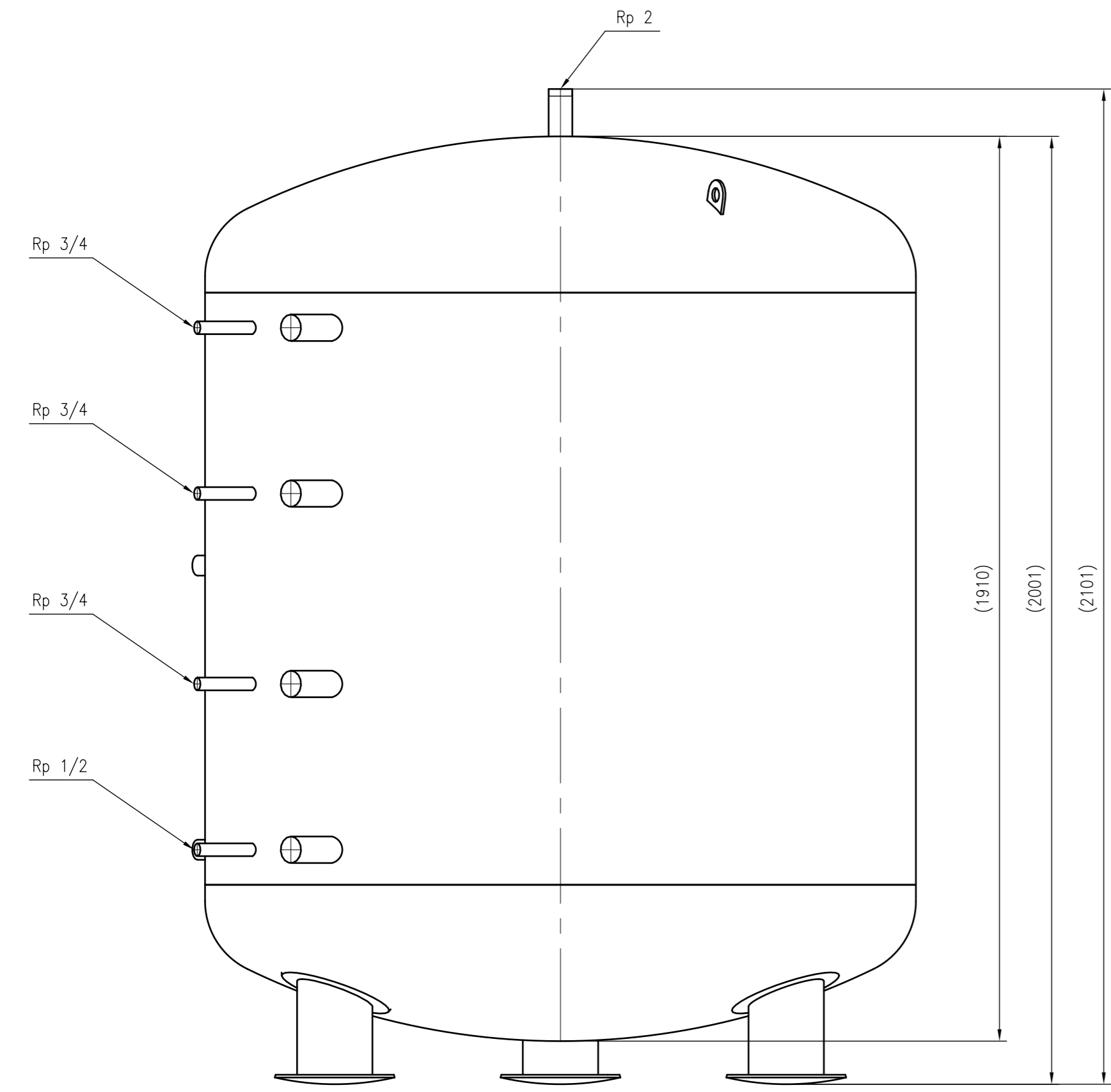
Side view
