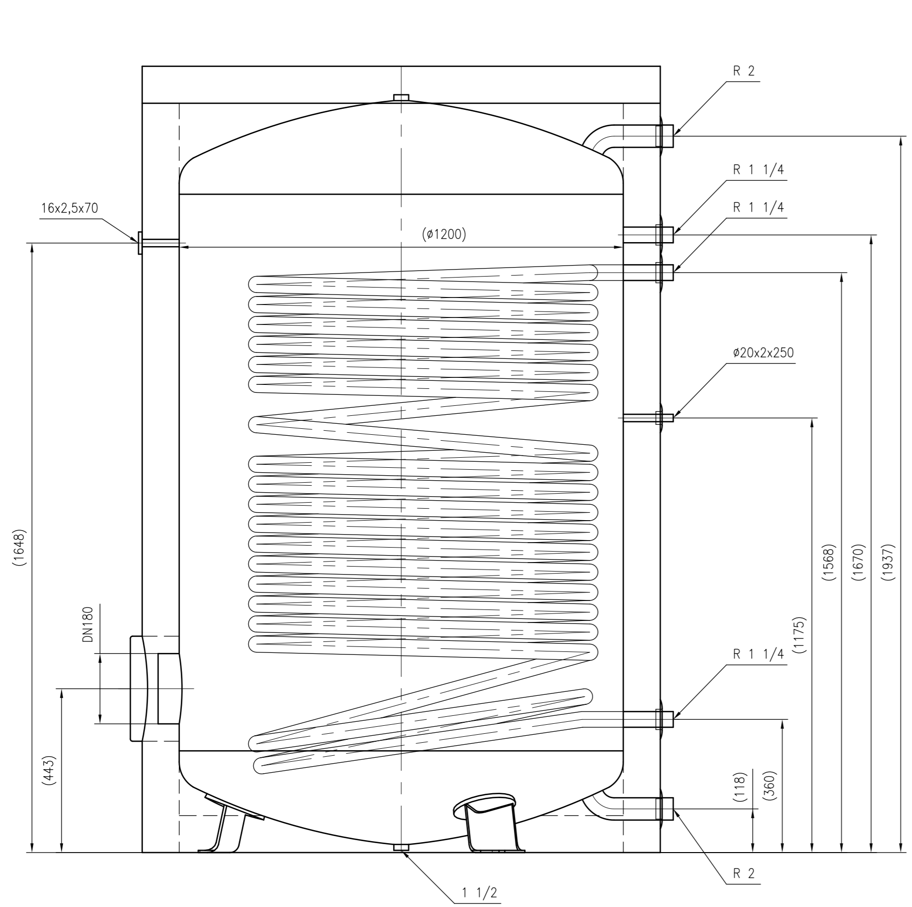
Side view
