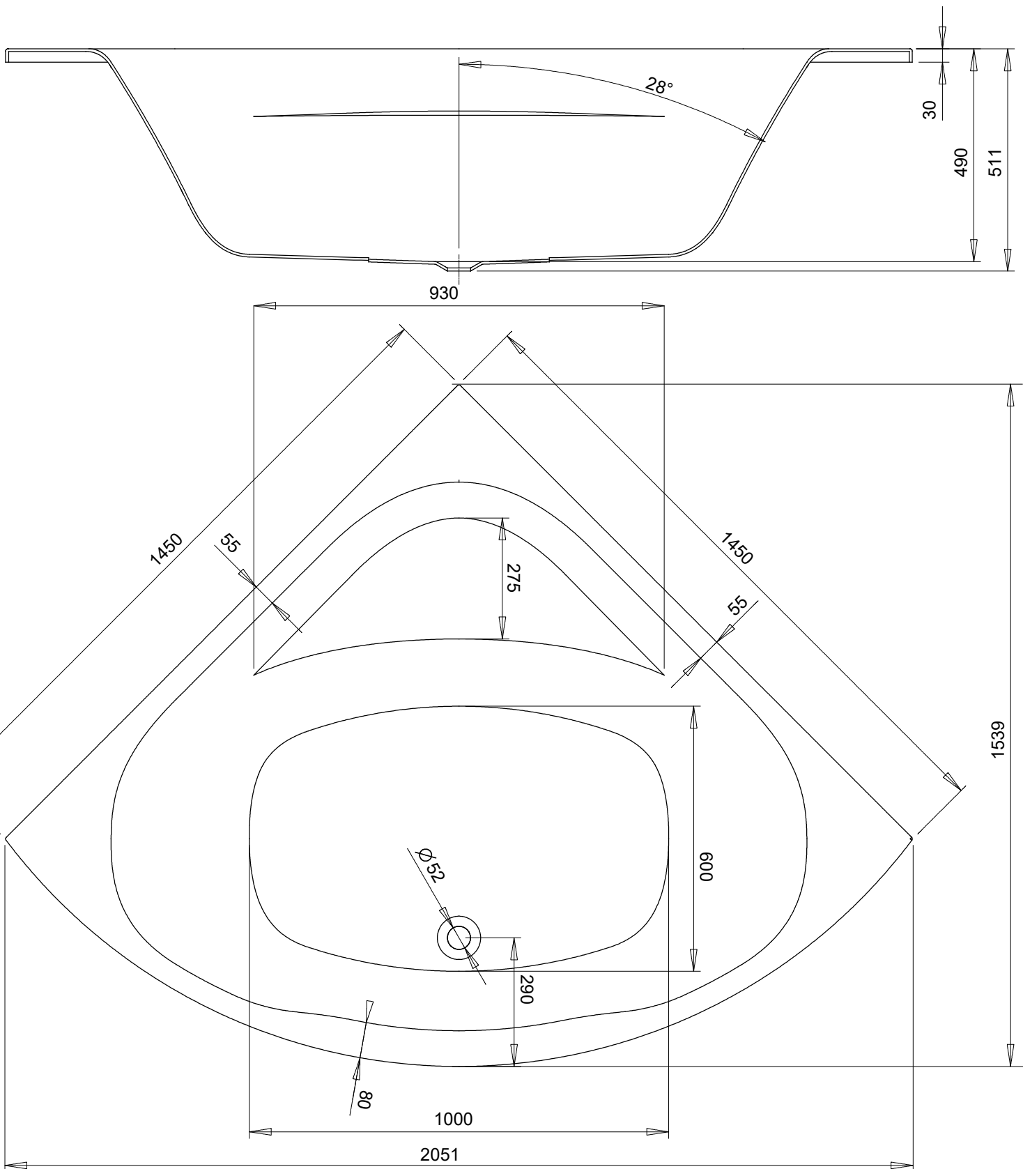
FORMAT Design Eckwanne 1450 x 1450 Art.-Nr.1330
