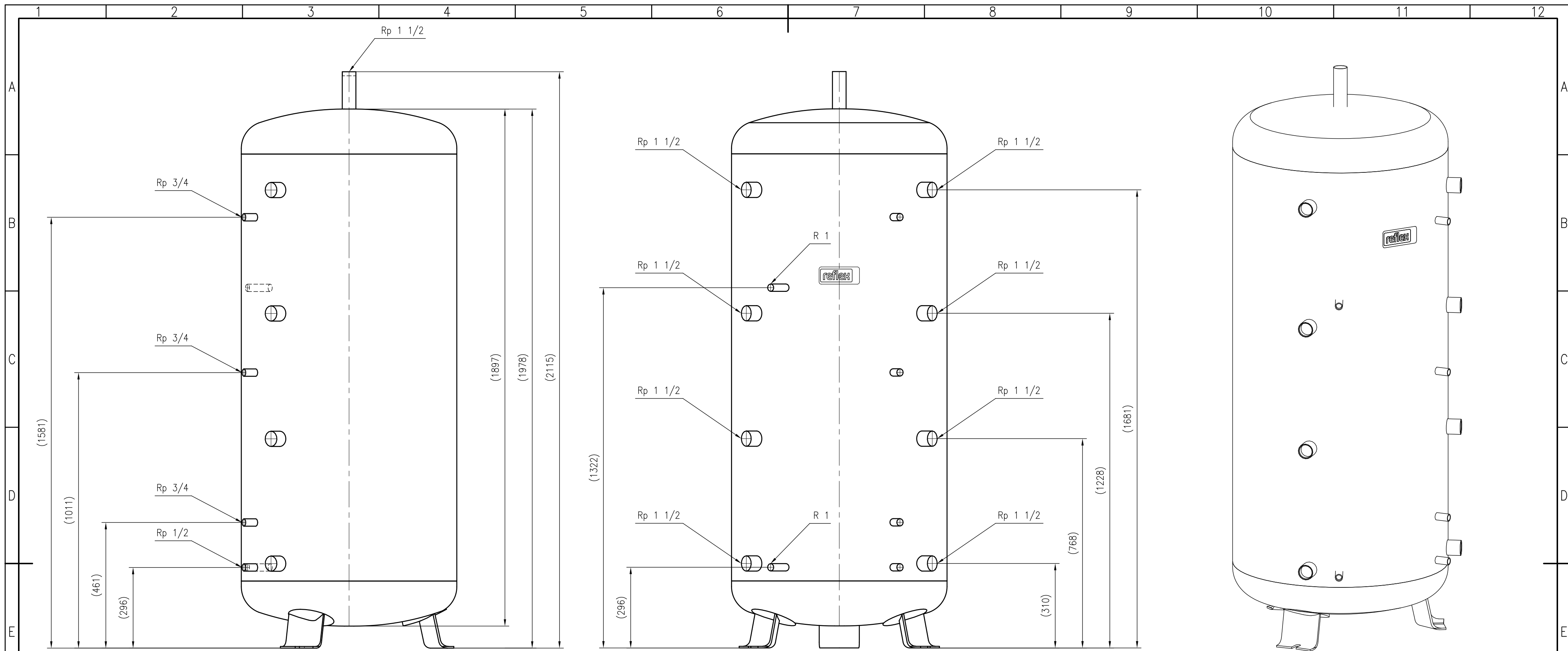
Side view
