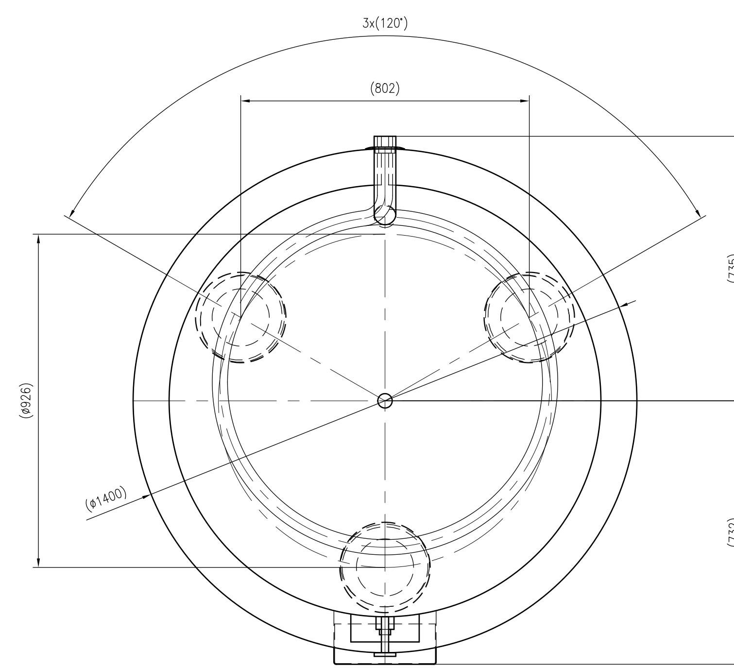
Top view
