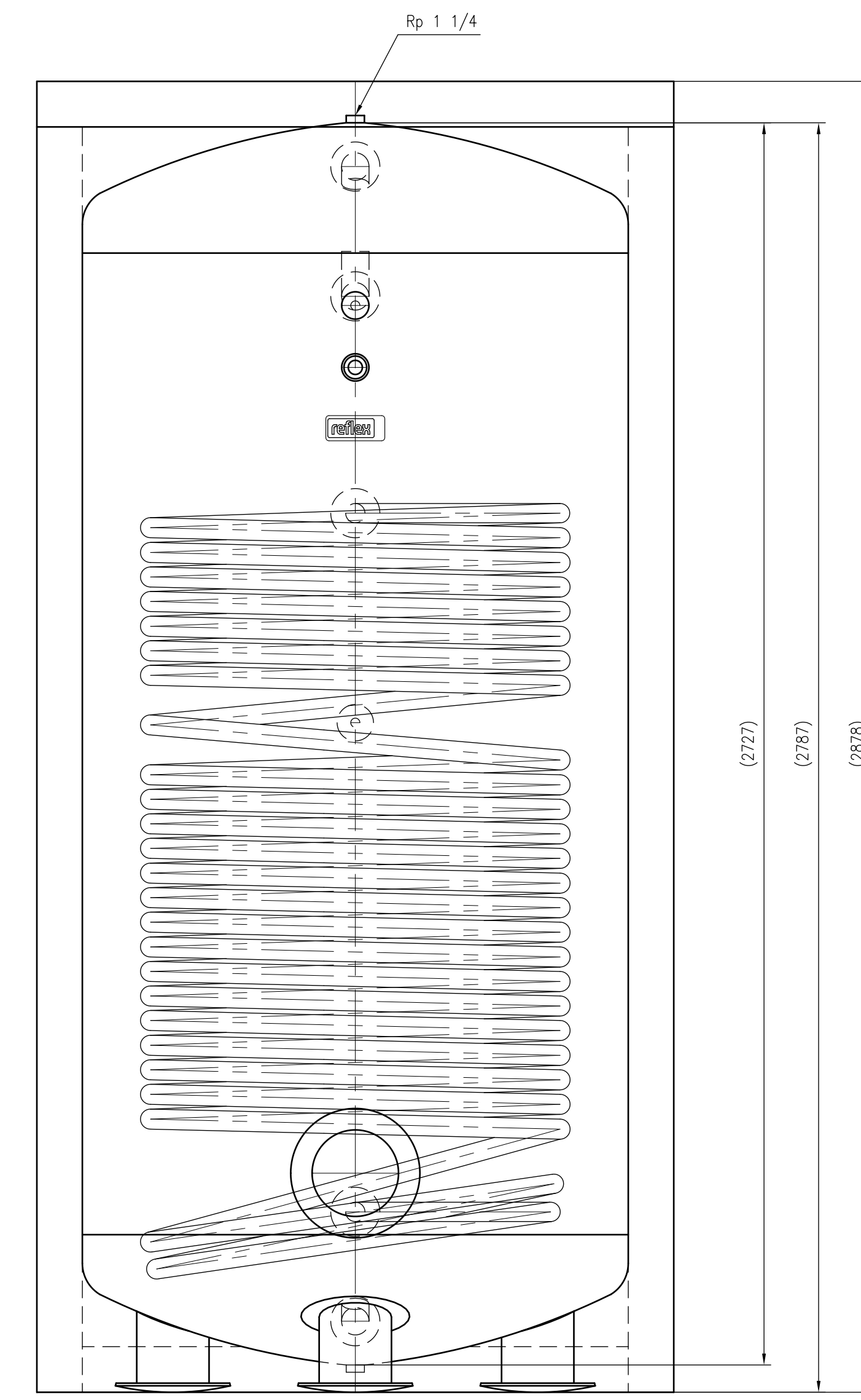
Front view
