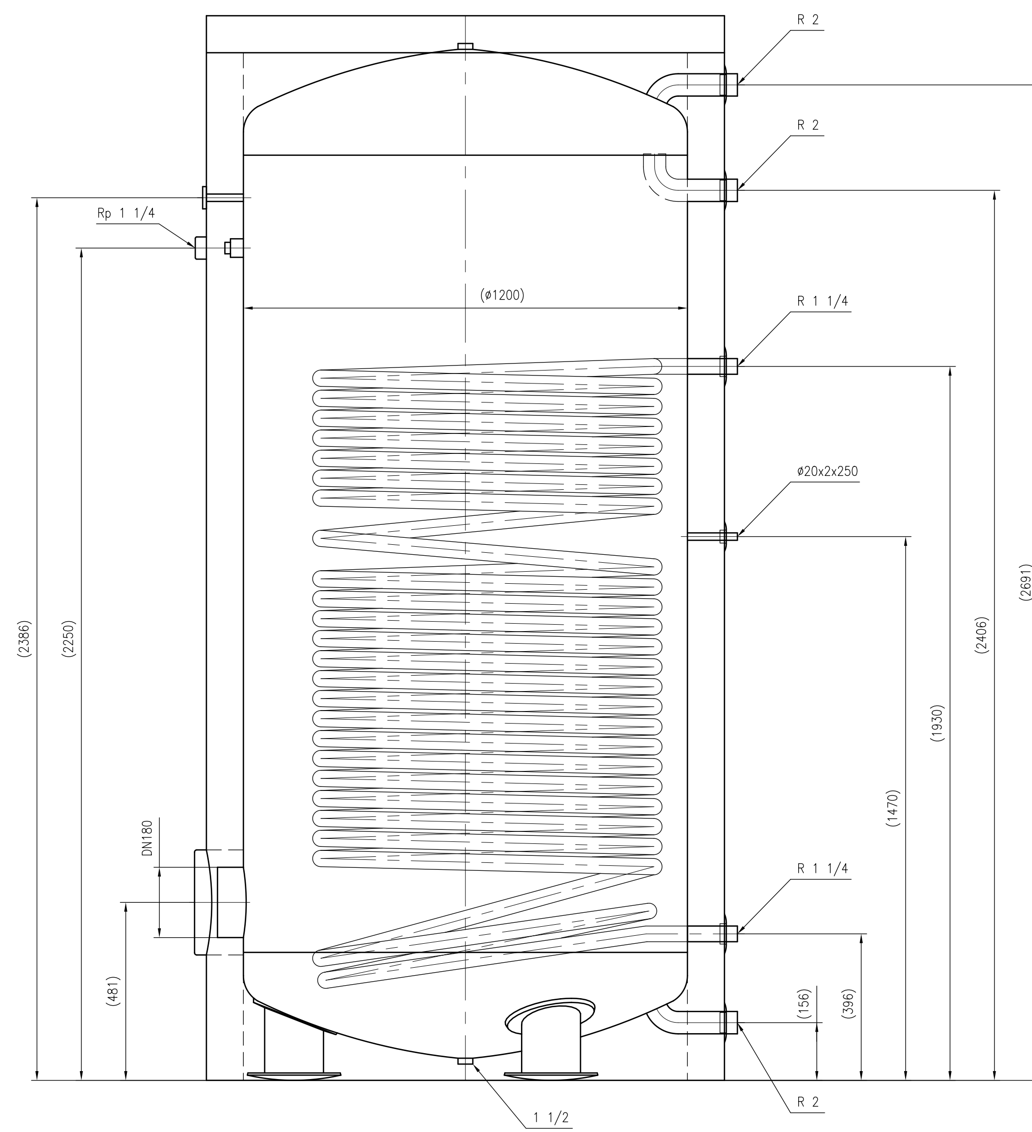
Side view
