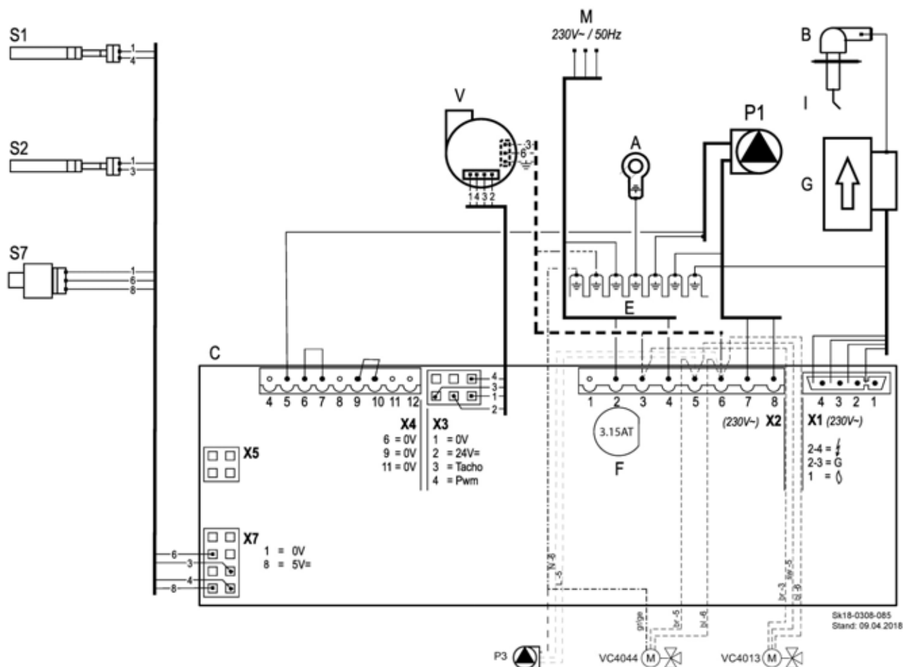
Abb. 30: Schaltplan ecoGAS ... Heizer
