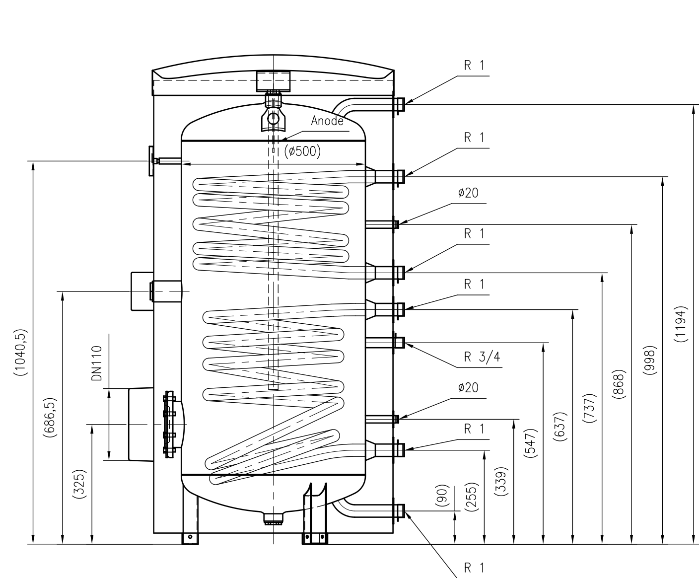
Side view
