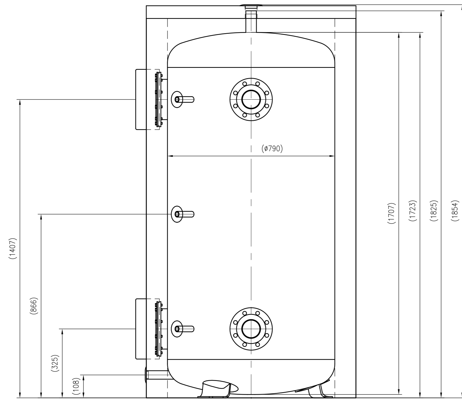
Side view
