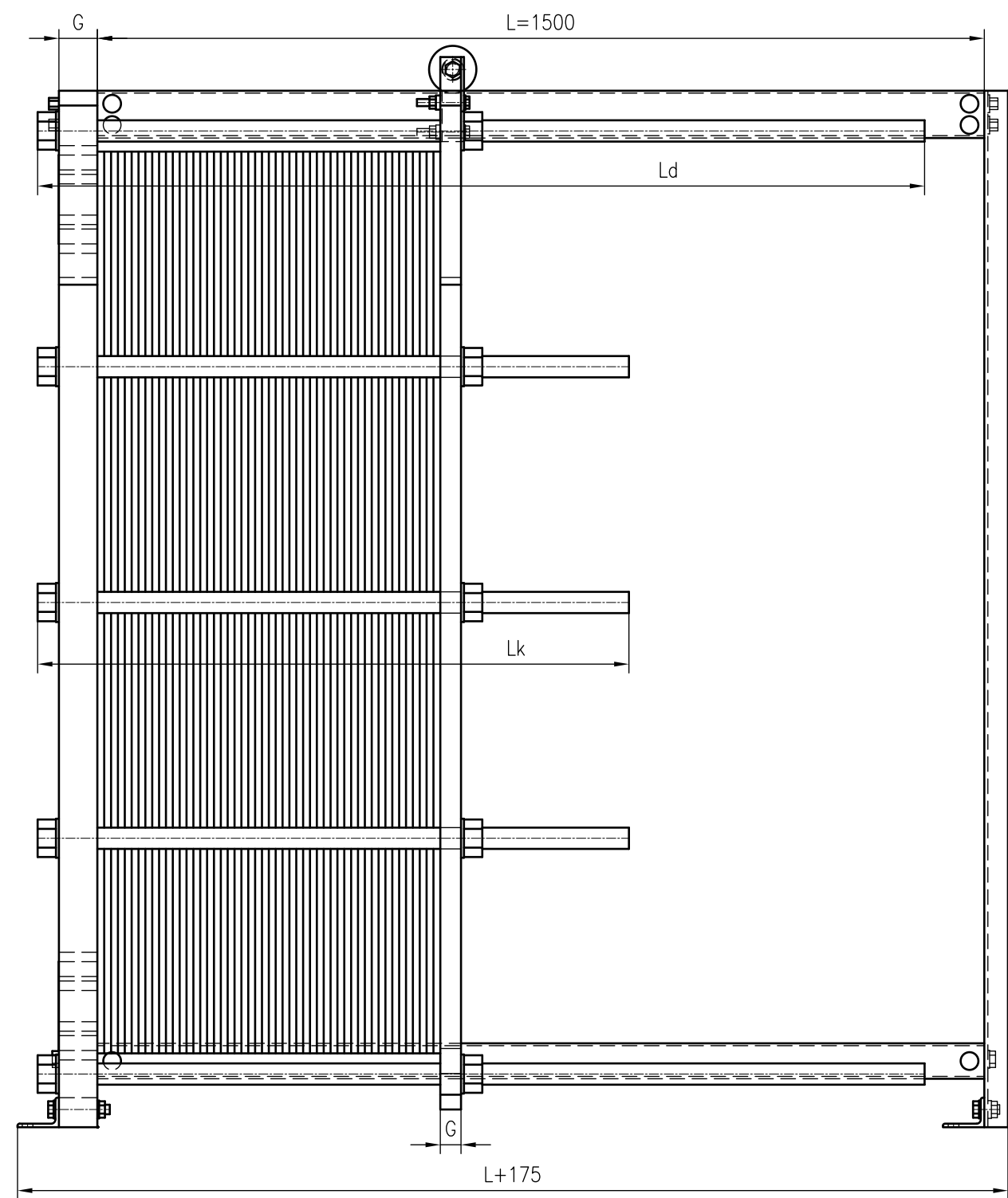
Side view
