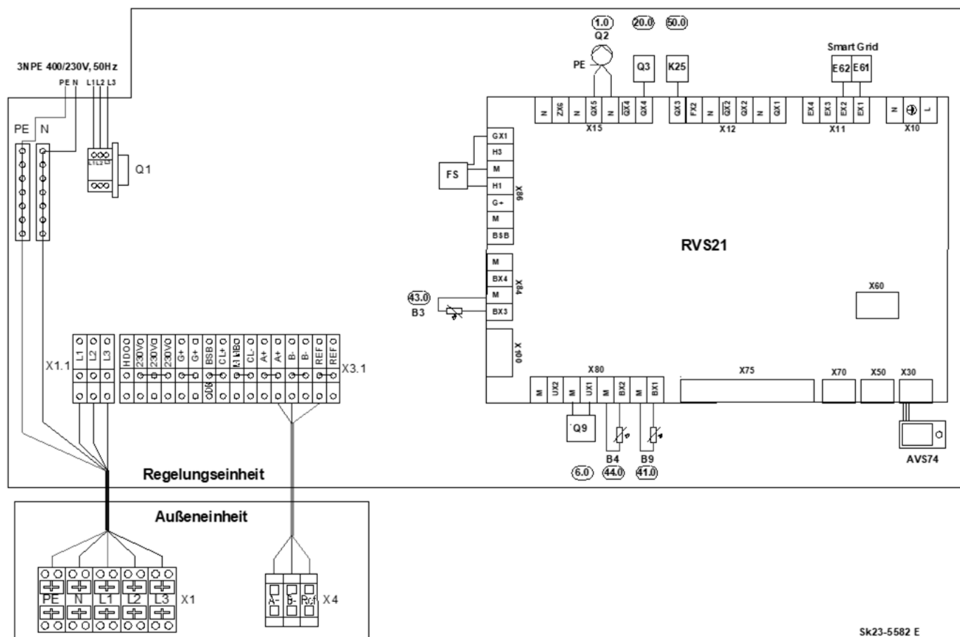
Abb. 29: Elektrik ecoWP Xe, UV, HK, Puffer, TWW
