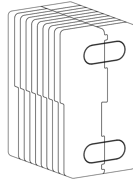
Isometric view
