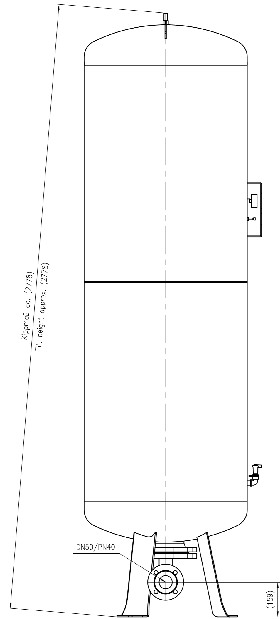
Side view
