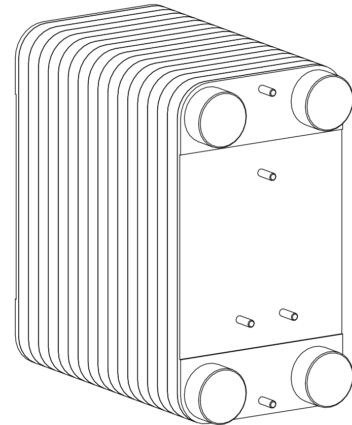
Isometric view
