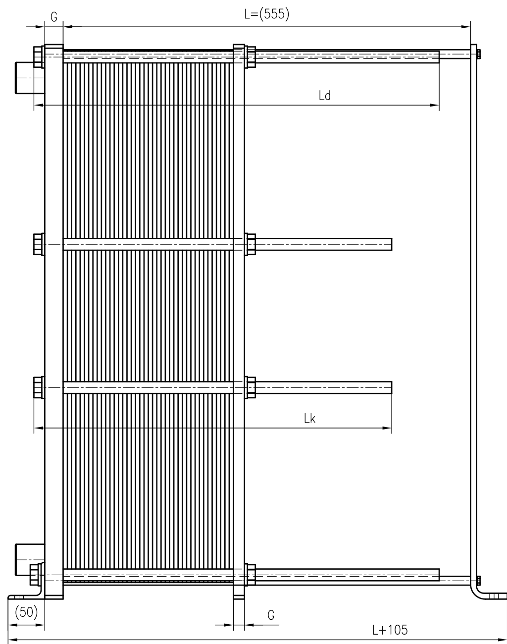
Side view
