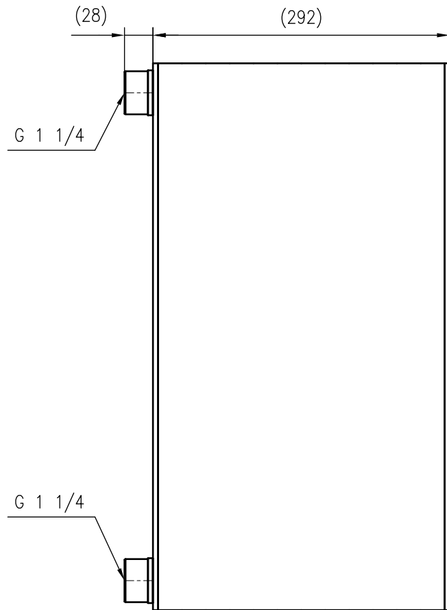
Side view
