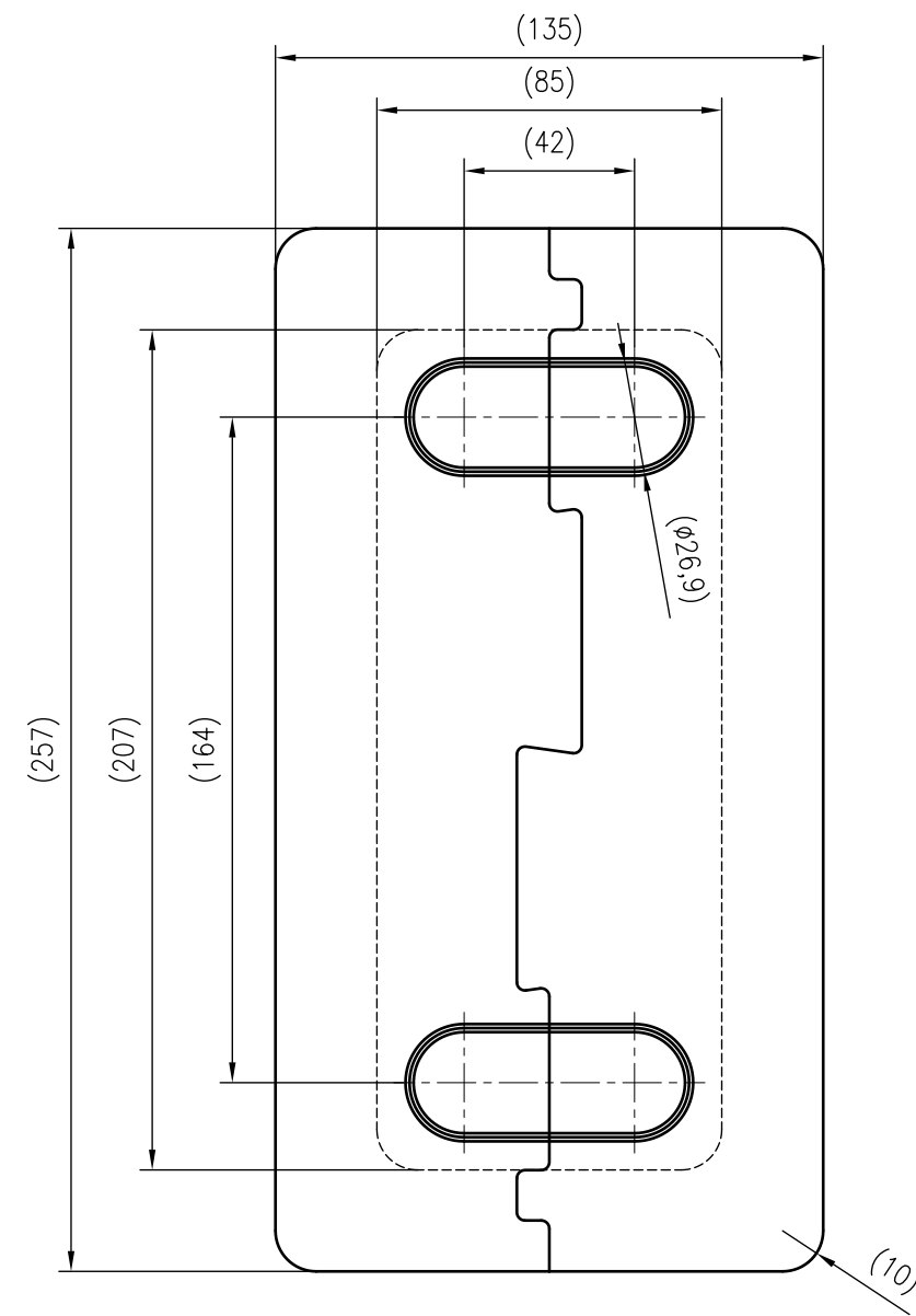
Front view
