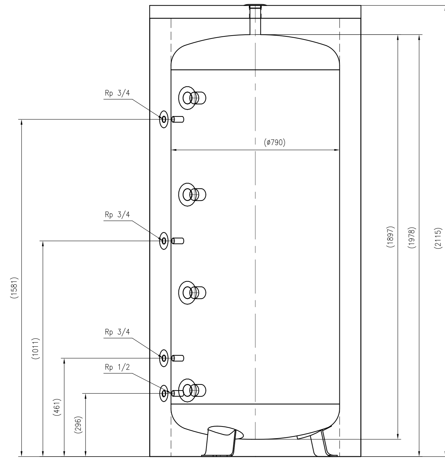
Side view
