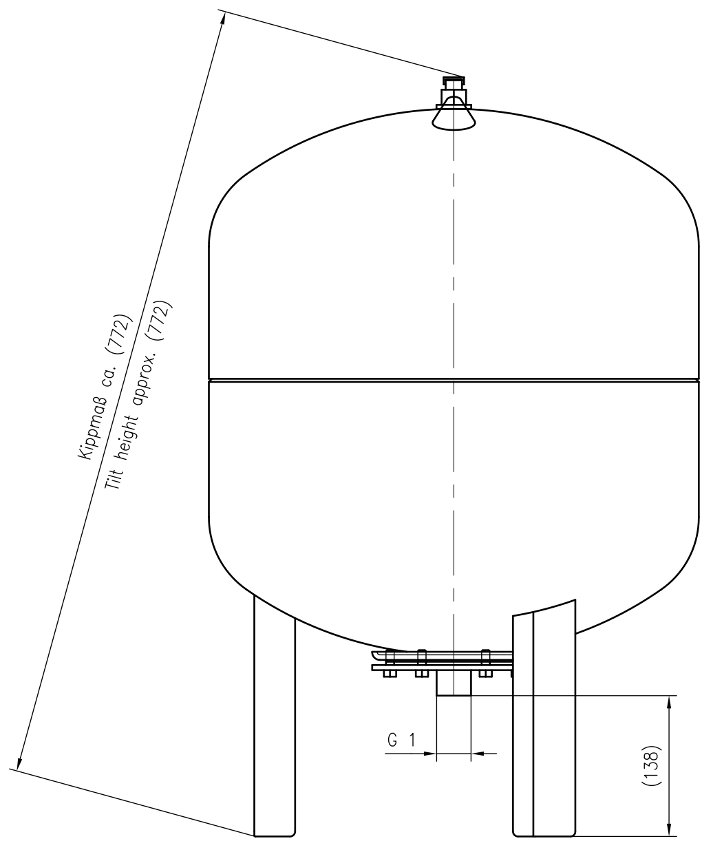
Side view
