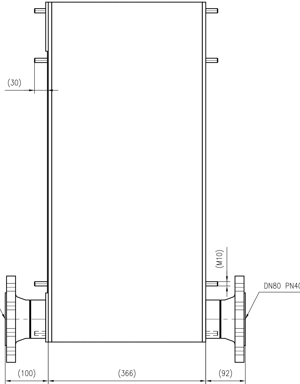
Side view
