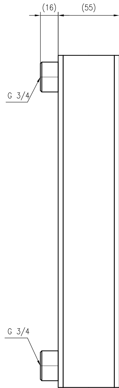
Side view
