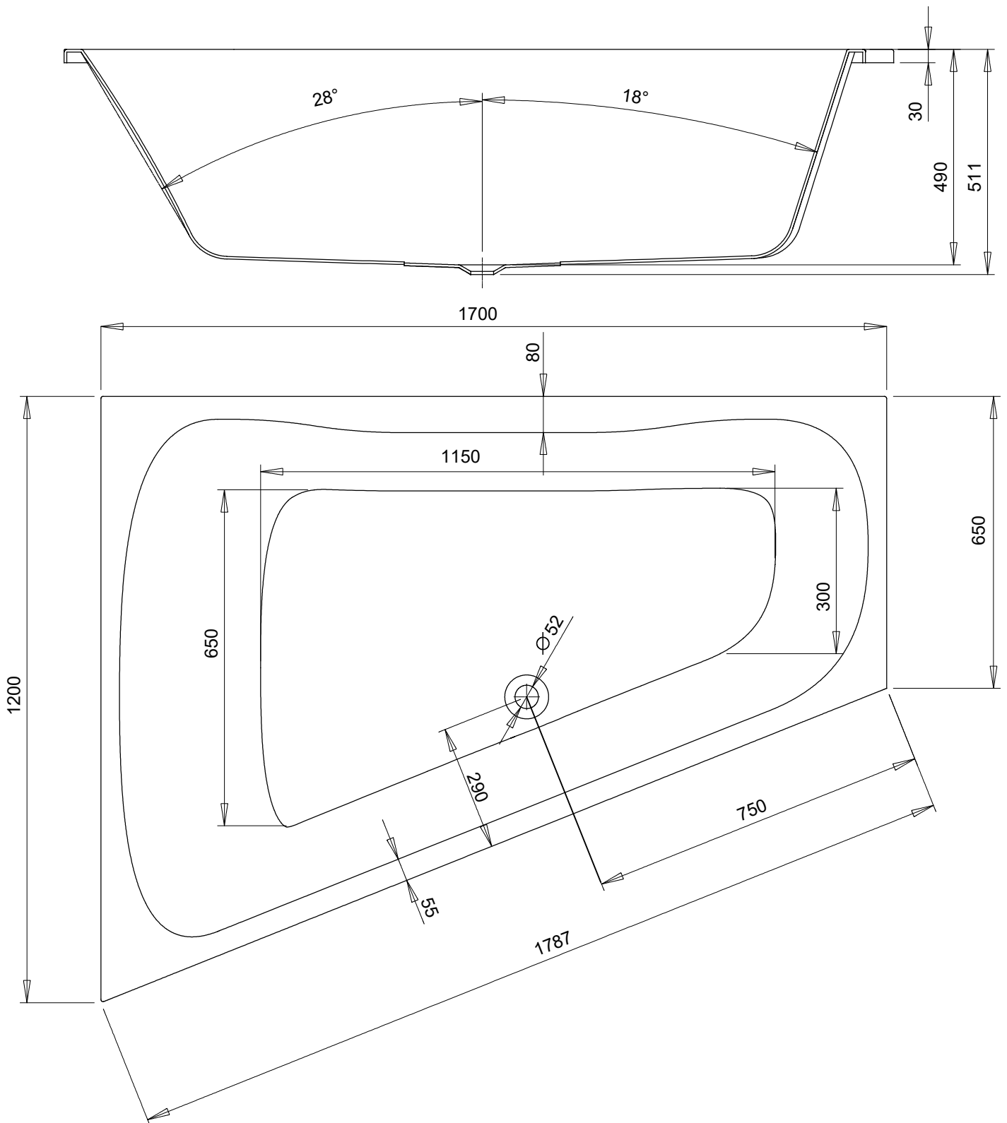
FORMAT Design Trapezwanne links 1700x1200x650
