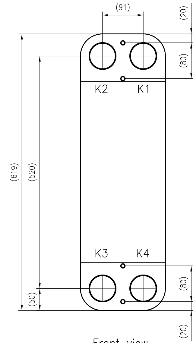
Front view
