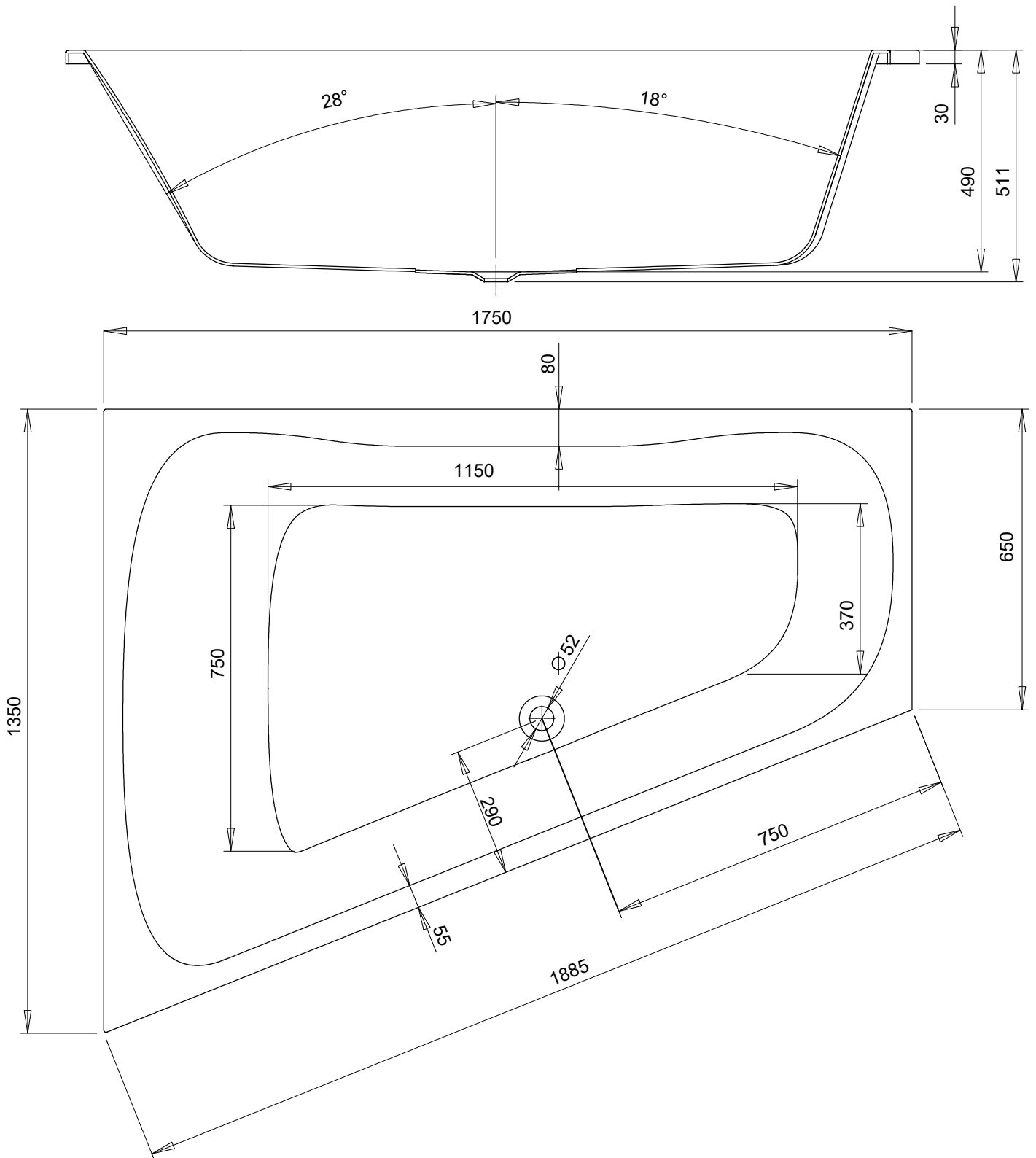
FORMAT Design Trapezwanne links 1750x1350x650 Art.-Nr.1334
