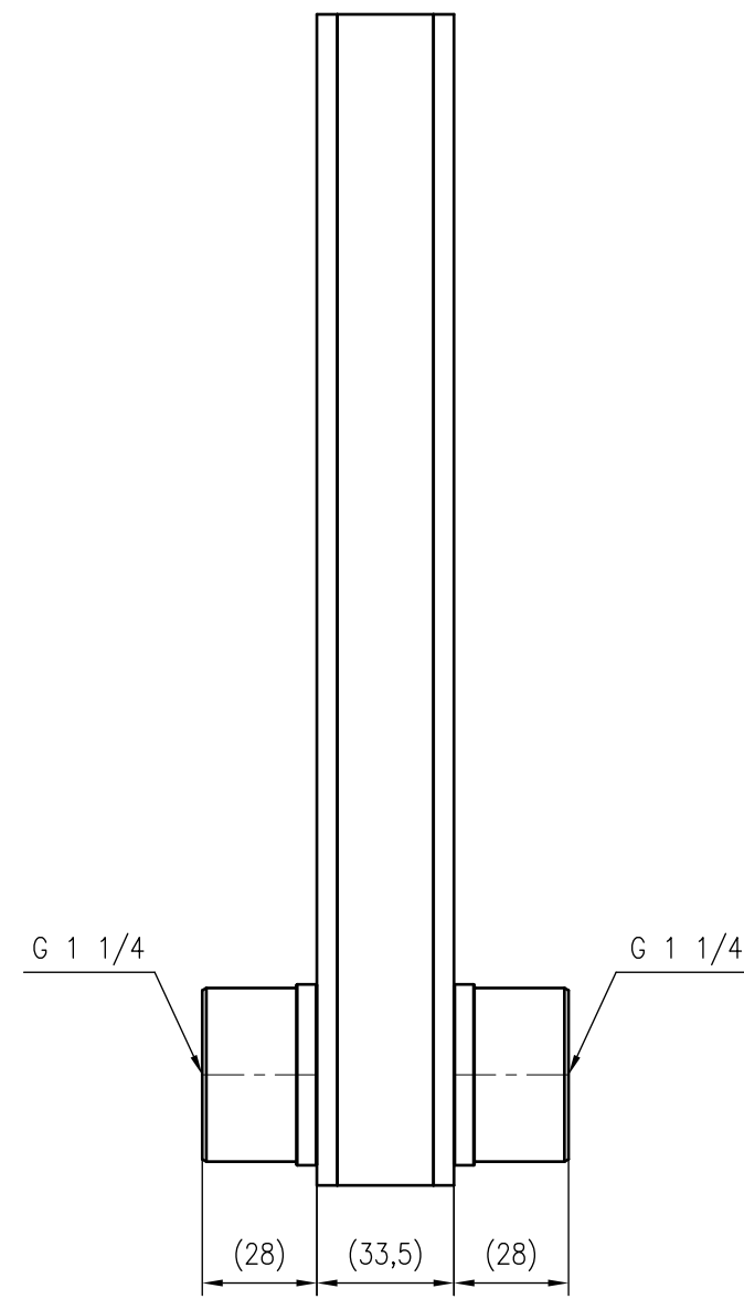
Side view
