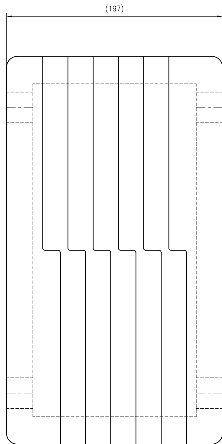
Side view
