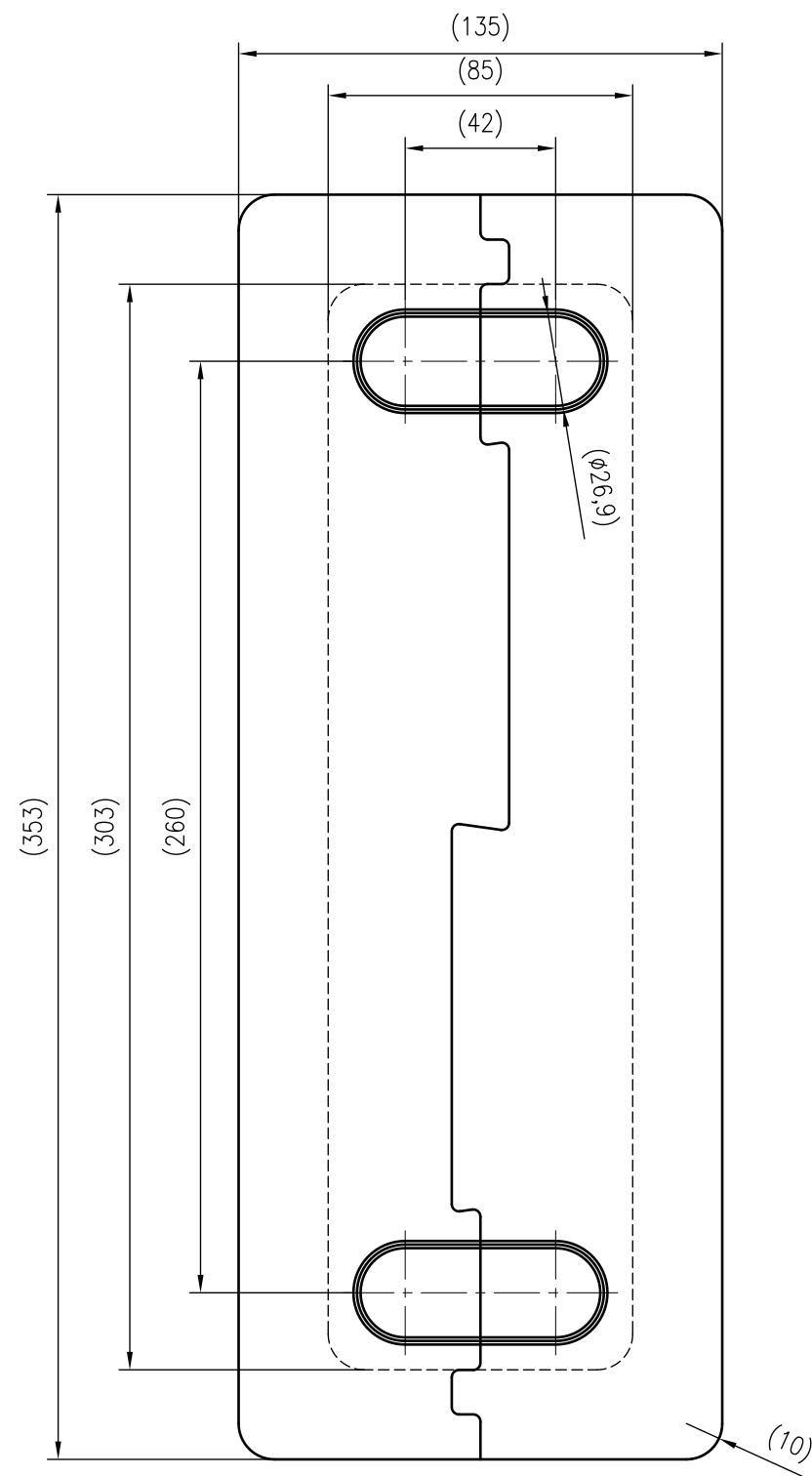
Front view
