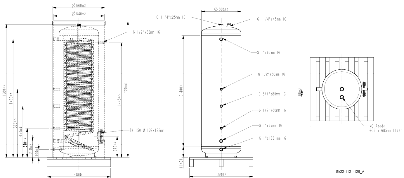
Abb. 20: THERAMAT WPS-300-1-F
