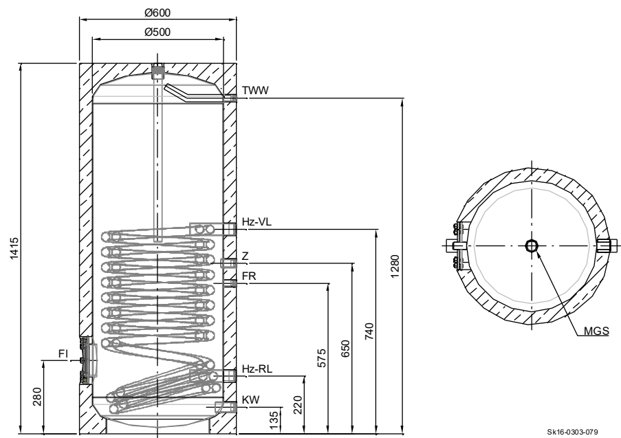
Abb. 7: THERAMAT EMH-200-1-F
