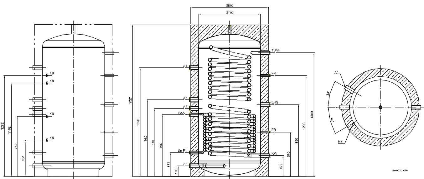
Abb. 15: THERAMAT SK-800-1
