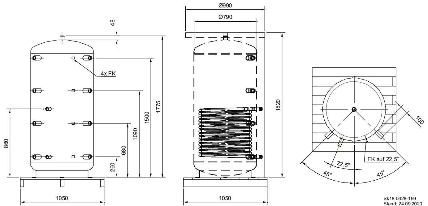
Abb. 19: THERAMAT SP-800-1
