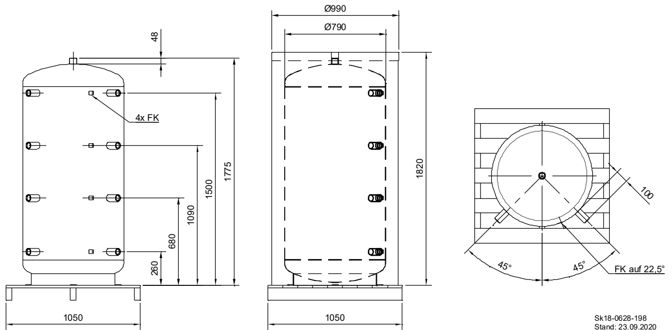
Abb. 18: THERAMAT SP-800-0
