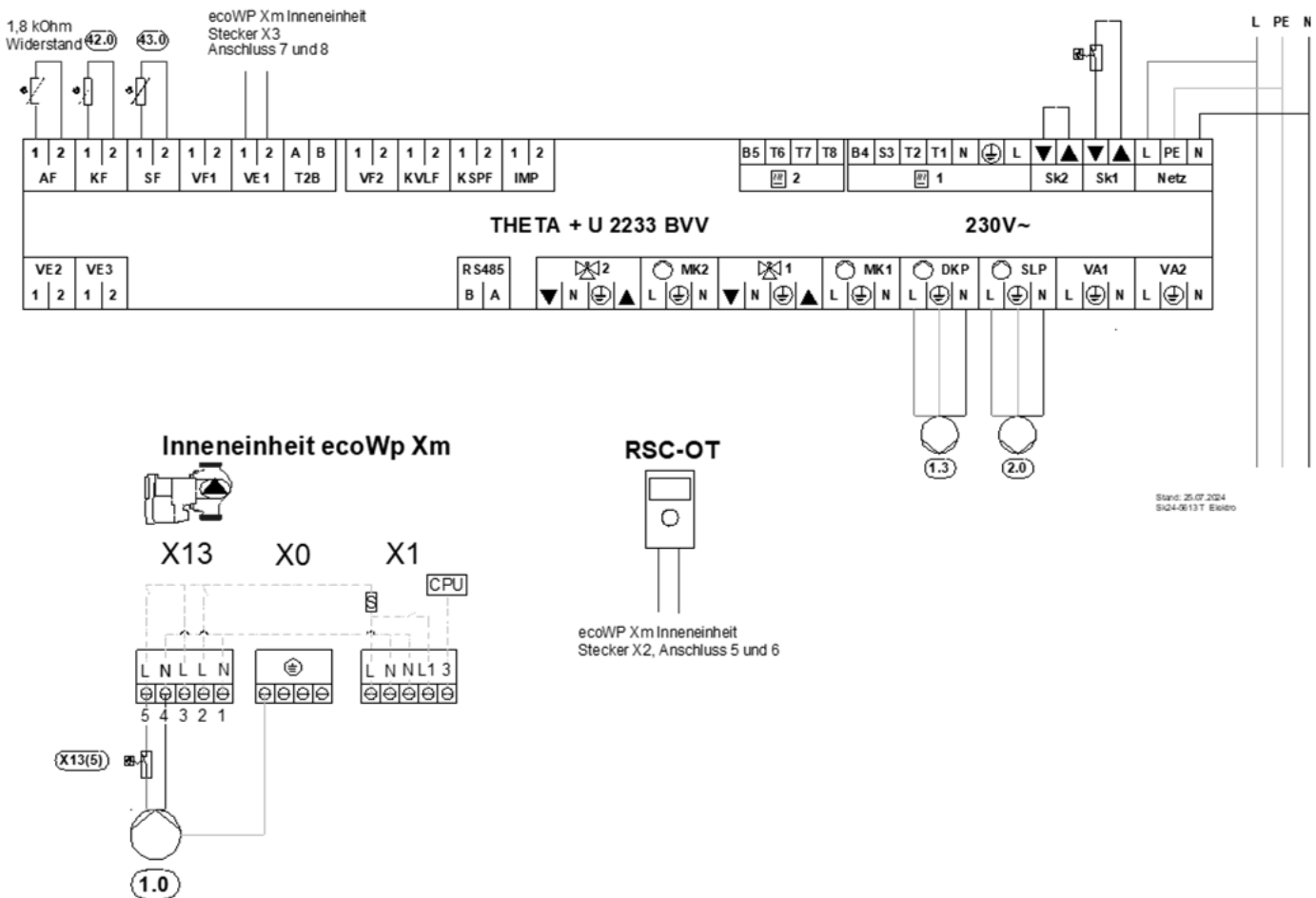
Abb. 39: Elektrik ecoDUO, ecoWP Xm, RSC-OT, UV, TWW, WW, HK
