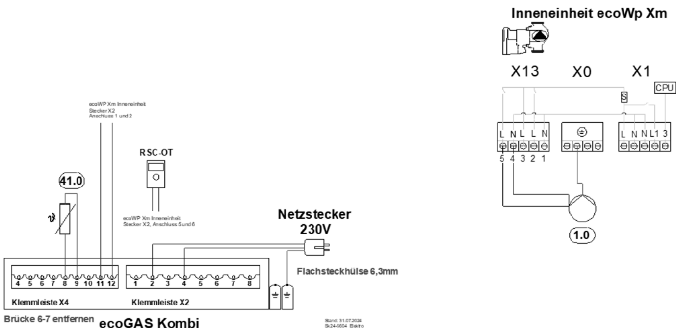
Abb. 37: Elektrik ecoGAS Kombi, ecoWP Xm, RSC-OT, WW, HK
