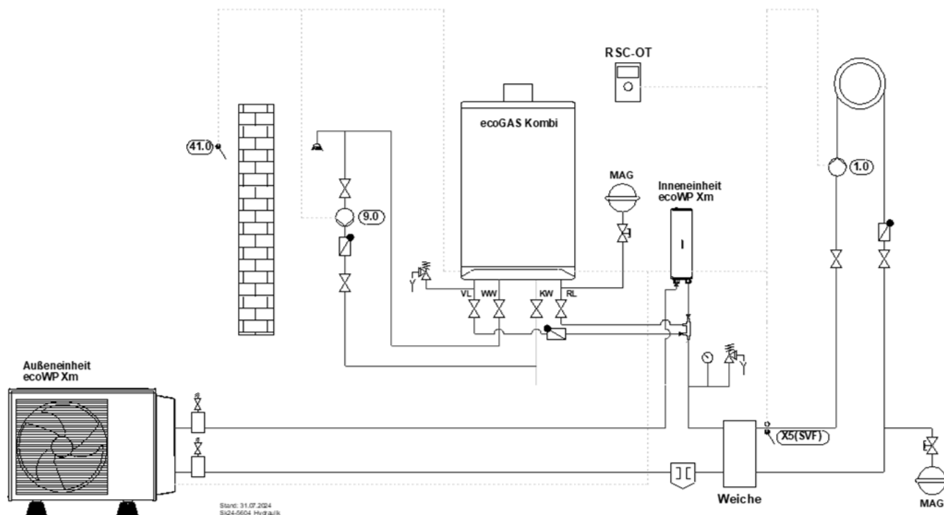
Abb. 36: Hydraulik ecoGAS Kombi, ecoWP Xm, RSC-OT, WW, HK
