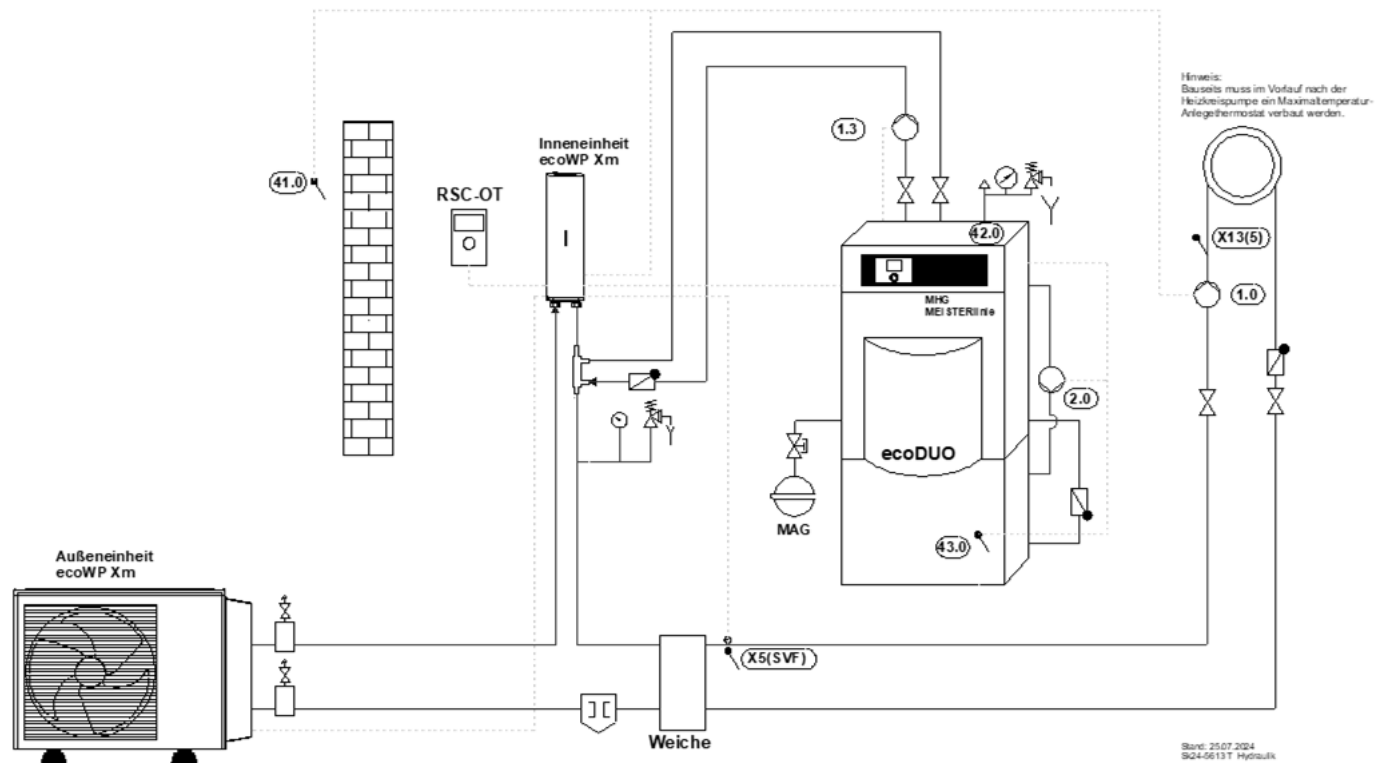
Abb. 38: Hydraulik ecoDUO, ecoWP Xm, RSC-OT, UV, TWW, WW, HK
