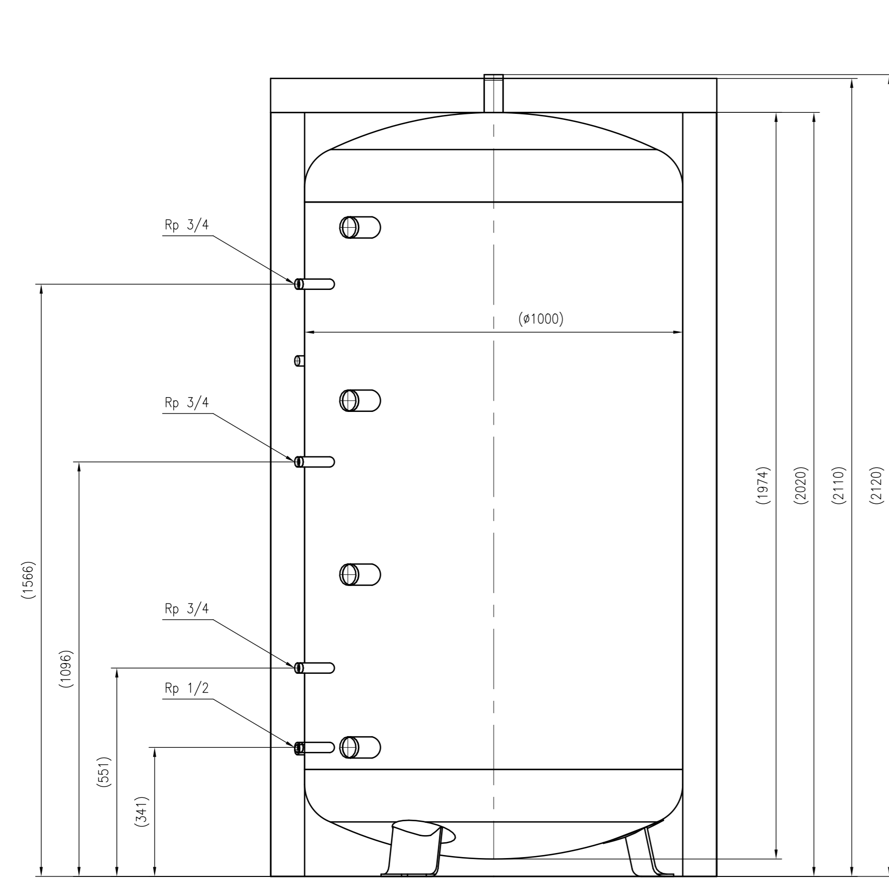
Side view
